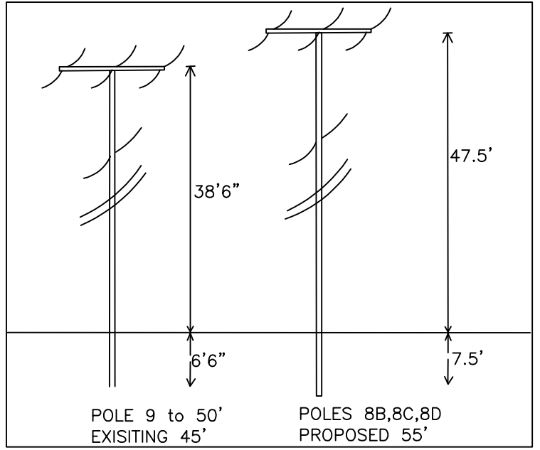
POLE HEIGHT VIEW
