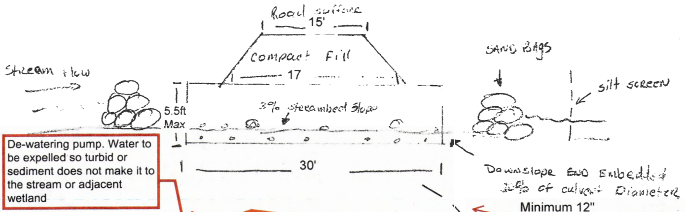
Plan View
