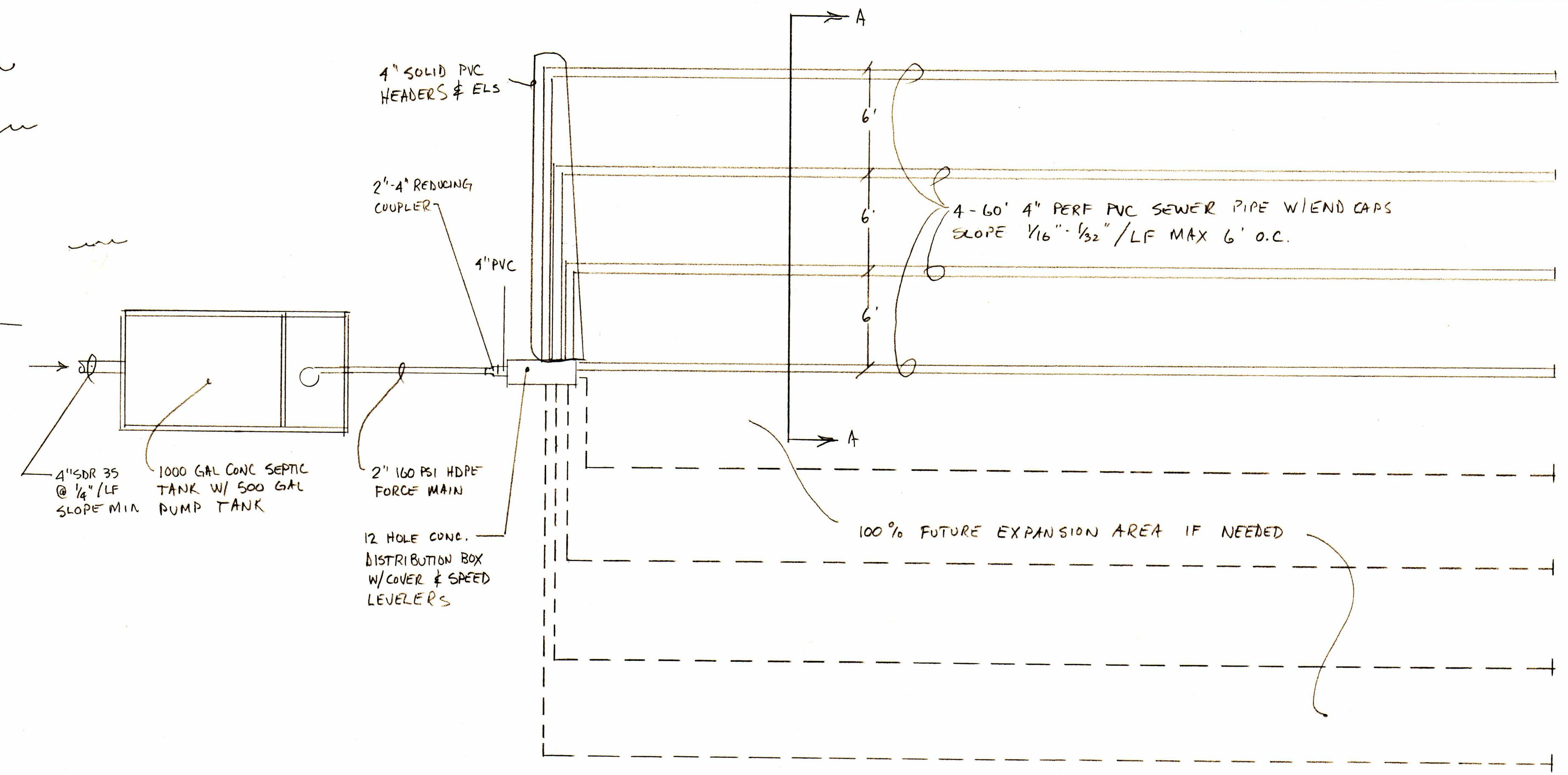
SHALLOW TRENCH ABSORPTION SYSTEM - SCHEMATIC PLAN VIEW SCALE 1" = 5'
