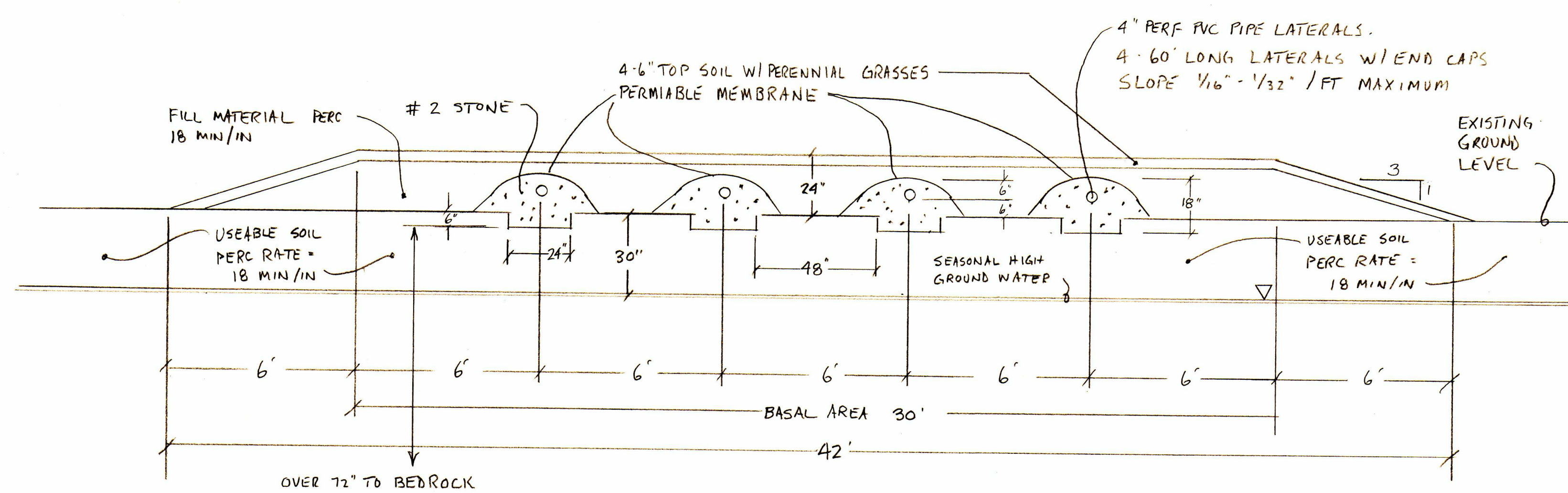
SHALLOW TRENCH ABSORPTION SYSTEM - SECTION VIEW A-A SCALE 1" = 3'
